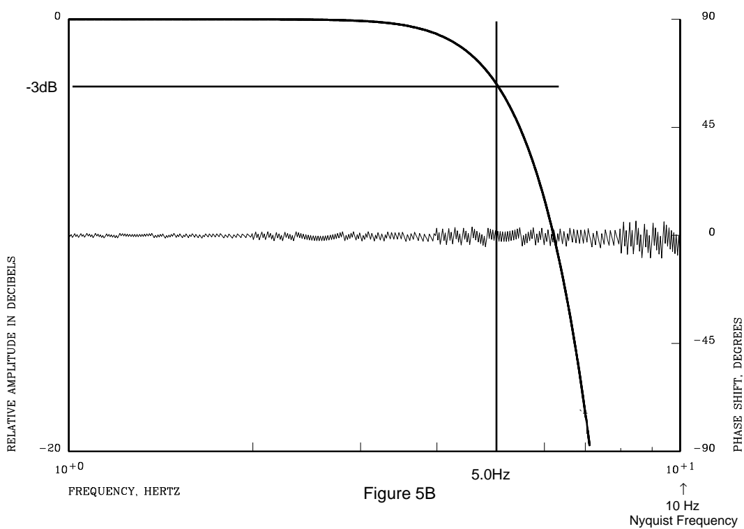
Figure 5: Amplitude response of Ormsby FIR filter used in the Reftek 24-bit digitizers of the IRIS/IDA IRIS-3 systems. 20 sps (BB) data. Gain is 0 dB at 0 Hz (DC). Note the different scales in the two figures above.
