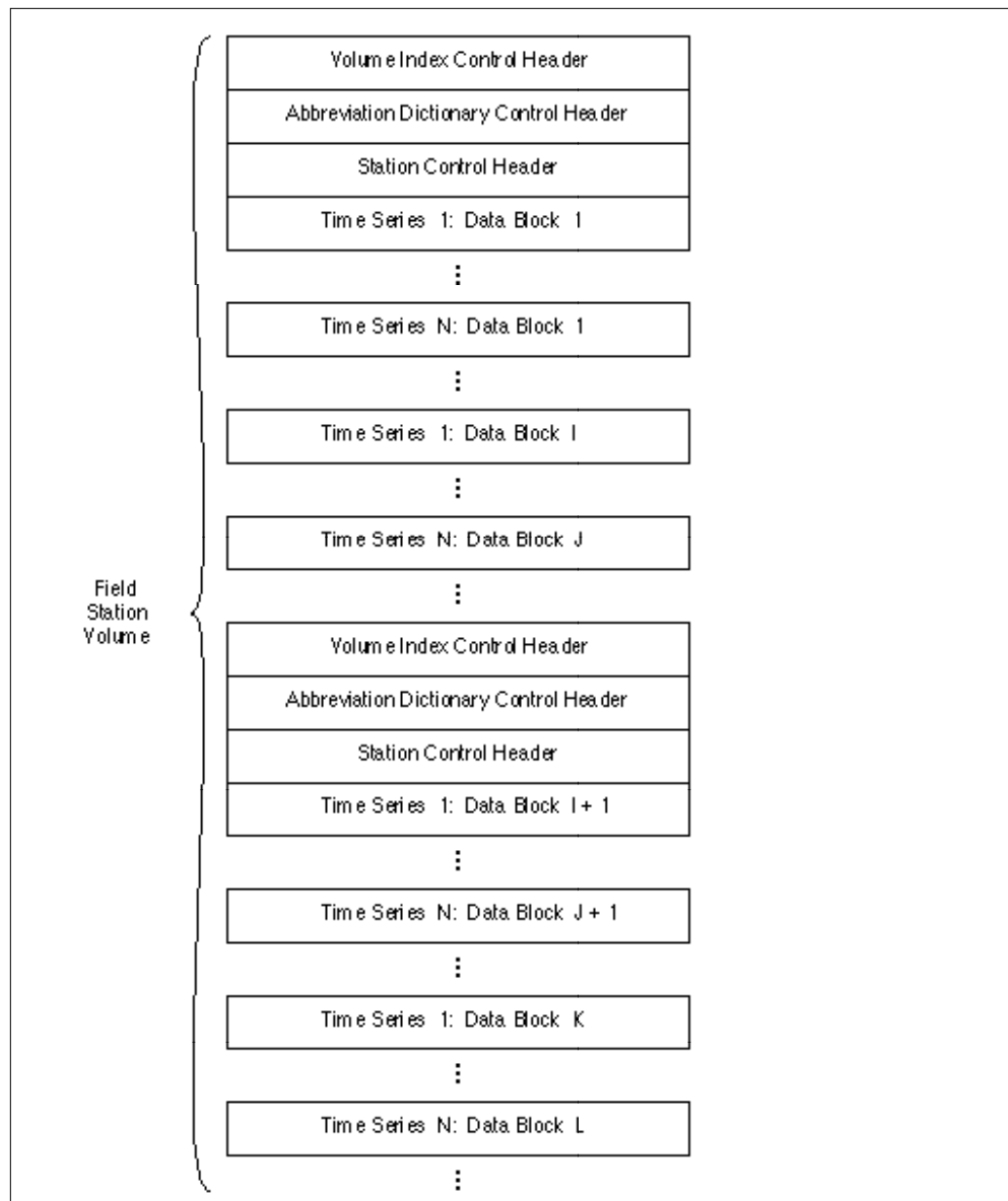
Figure 9: Organization of a Field Station Volume
