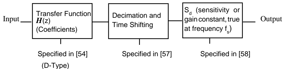
Figure 8: Example Digital Stage Using Coefficients Representation
