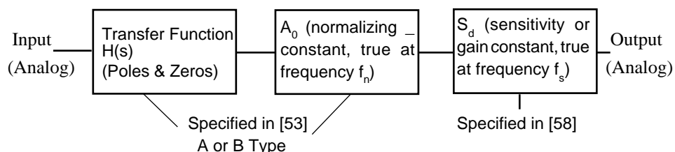
Figure 6: Example Analog Stage Using Poles and Zeros Representation
