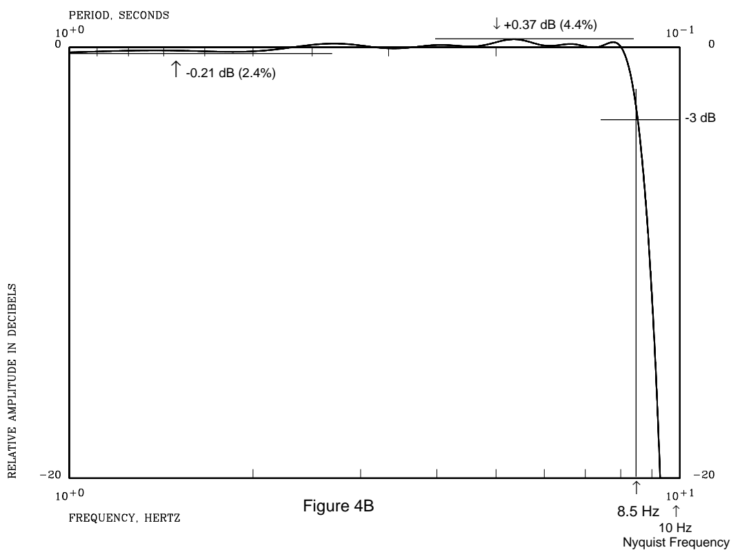
Figure 4: Amplitude response of combined FIR filters used in Q380 and Q680 model digitizers built by Quanterra, Inc. for 20 sps (BB) data. Gain has been normalized to 0 dB at 0 Hz (DC).
