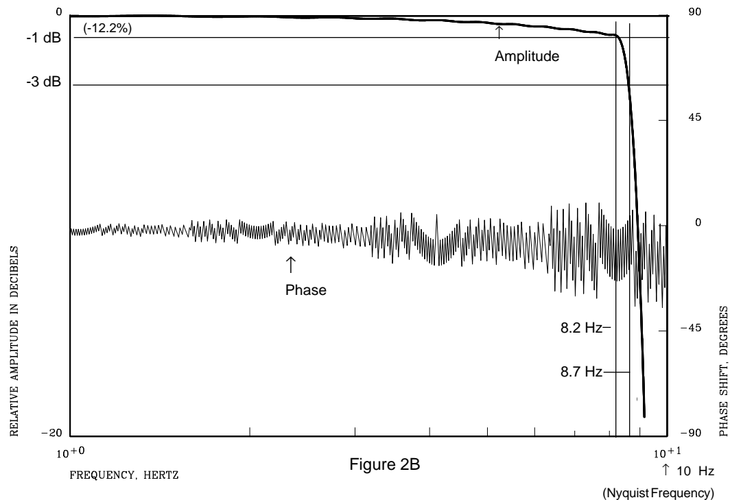
Figure 2: Amplitude response of combined FIR filters used in Martin-Mariette digitizers of IRIS/USGS IRIS-2 systems, 20 sps (BB) data. Gain has been normalized to 0dB at 0 Hz (DC). Note the different scales in the two figures above.
