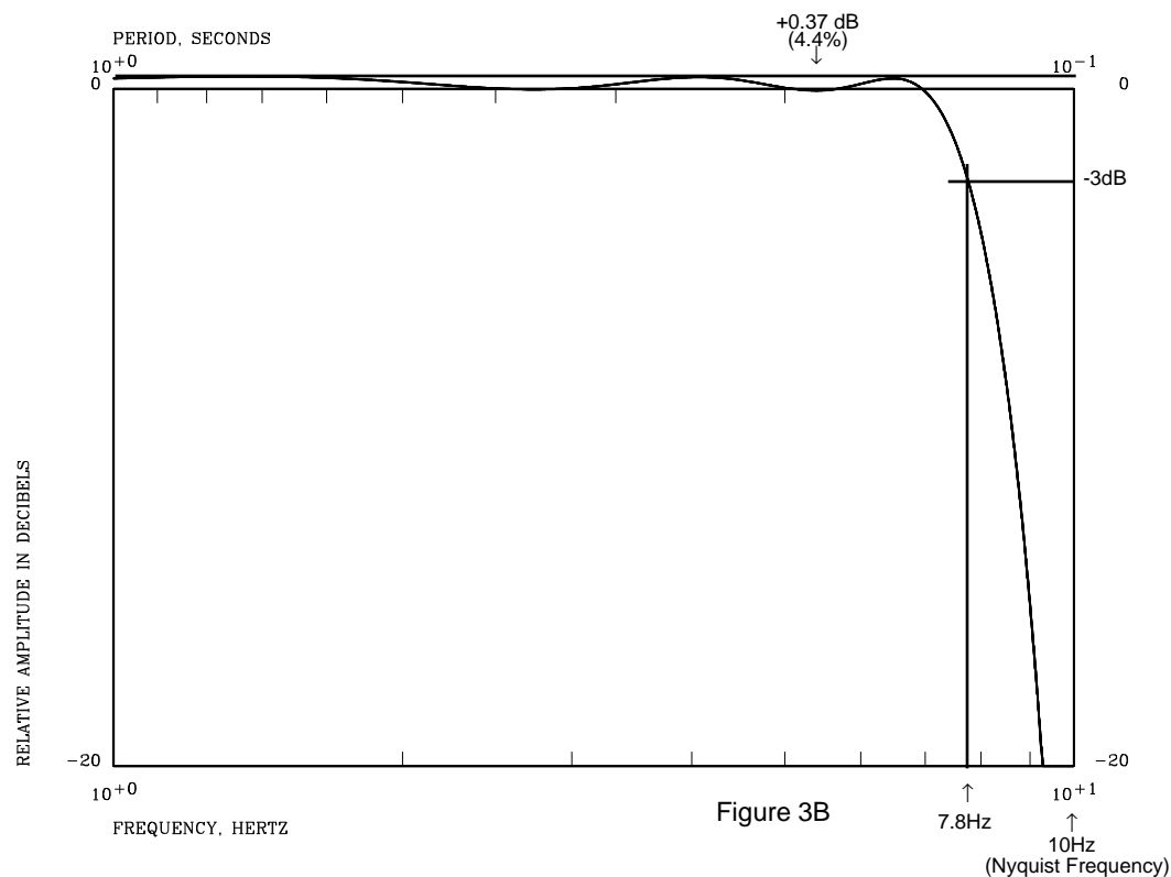
Figure 3: Amplitude response of combined FIR filters used in “Quantagrator” model digitizers built by Quanterra, Inc. for 20 sps (BB) data. Gain has been normalized to 0db at 0Hz (DC).
