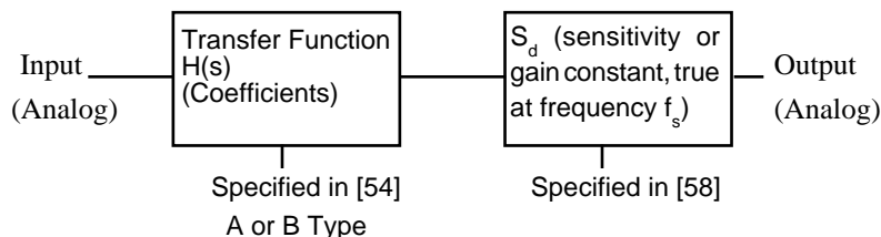
Figure 7: Example Analog Stage Using Coefficients Representation
