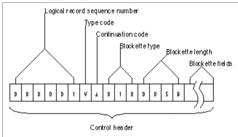
Figure 10: Beginning Fields of a Control Header
