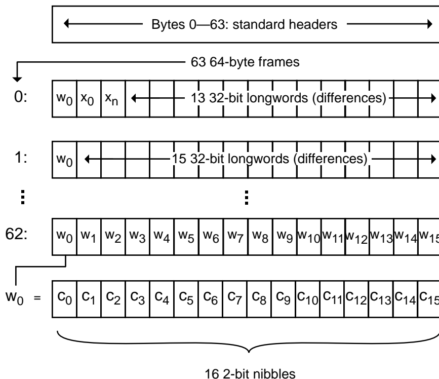
Figure 13: Compressed Data Format
